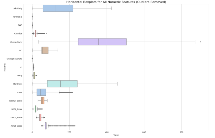
Fig. 8: Dataset after Removing Outliers.
