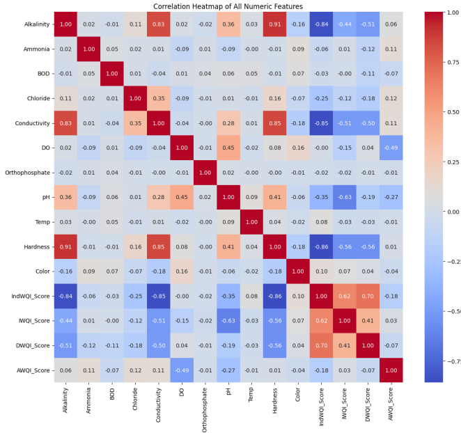
Fig. 6: Feature Correlation with WQI's of the Modified Dataset
