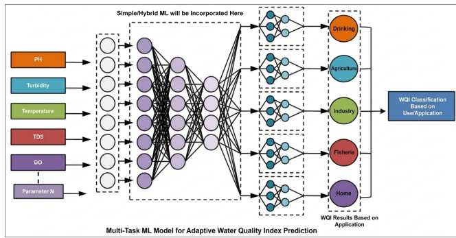
Fig. 17: Tentative Multi-task ML Framework for Milestone 3
