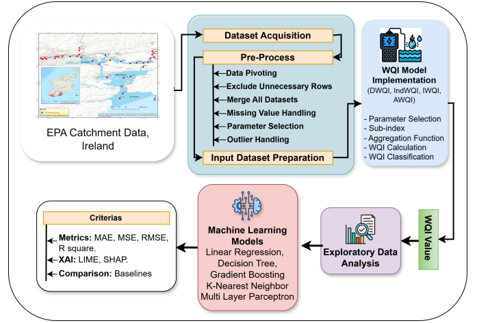
Fig. 12: Overall pipeline of the study design.
