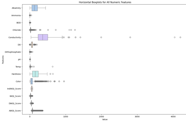
Fig. 7: Dataset before Removing Outliers.
